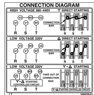
Connection Diagram
