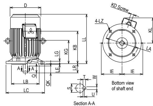
Outline Drawing
